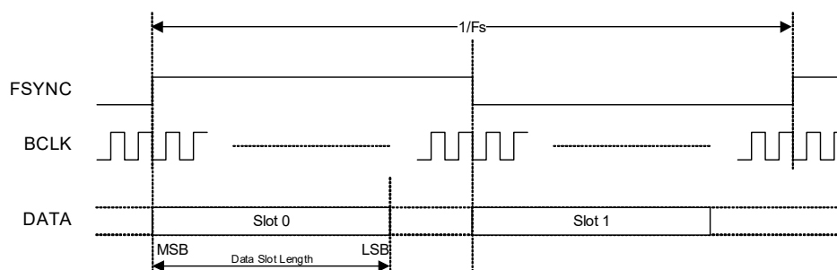
Figure 4-8. Left-Justified Data Format
