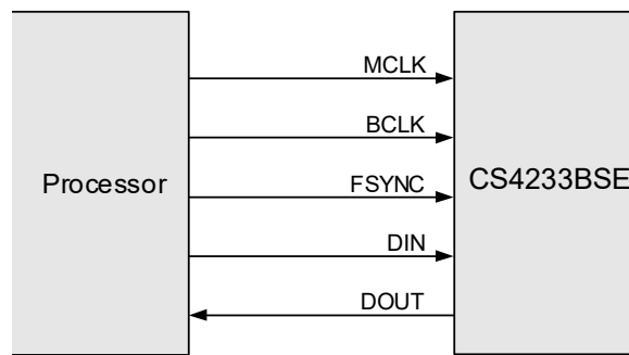
Figure 4-4. Secondary Mode, MCLK Clocking Source
