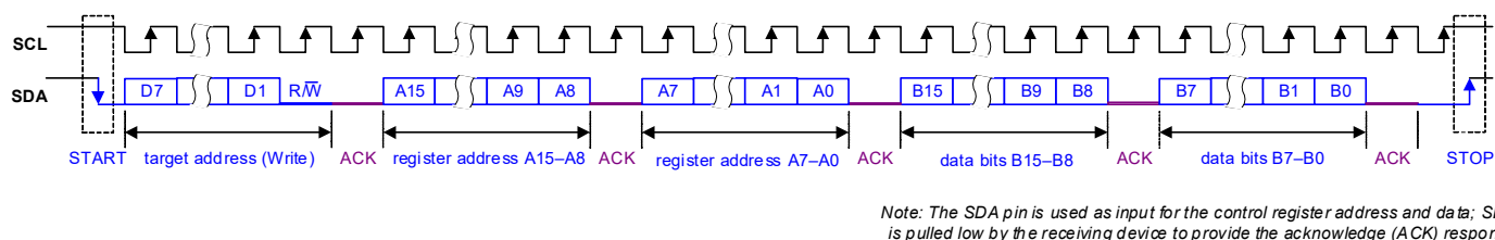
Figure 4-17. Control Interface I 2 C Register Write
