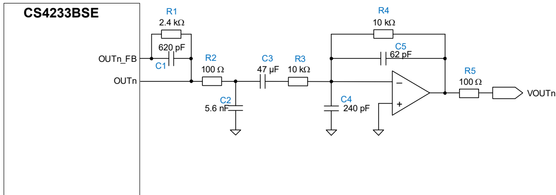
Figure 5-3. Example Active Line Driver Circuit
