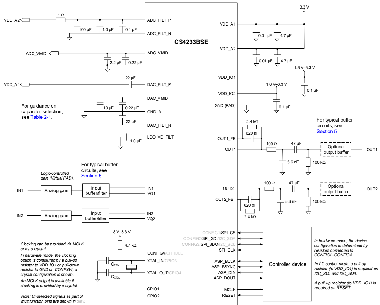
Figure 2-1. Typical Connections
